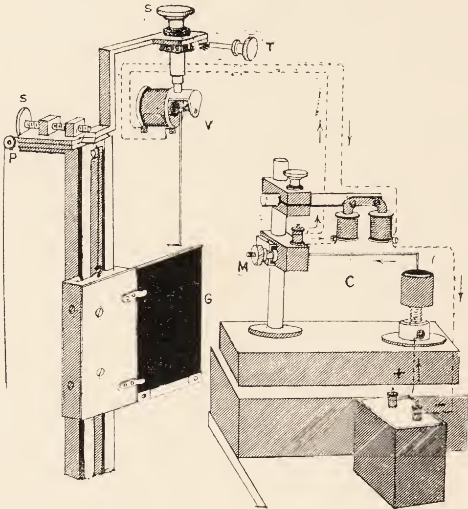
FIG. 10.—Upper part of the Resonant Recorder. Thread from clock, not shown, passes over pulley (P), letting down recording smoked glass plate (G) ; C, coercing reed which by its vibration sets recorder (V) in sympathetic vibration. The axis of recorder (V) is supported perpendicularly at centre of circular end of magnet. S S', adjusting screws ; M, micrometer ; T, tangent screw.
